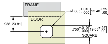
MOUNTING DIMENSIONS
