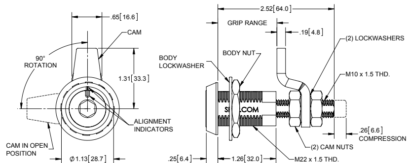
MOUNTING DIMENSIONS
