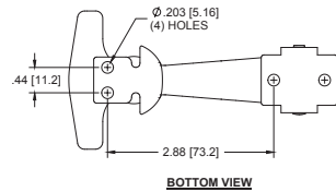
LATCH WITH SHORT KEEPER
