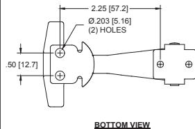
LATCH WITH SHORT KEEPER
