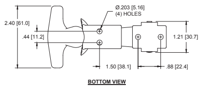
LATCH WITH LONG KEEPER
