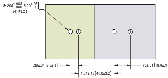
MOUNTING DIMENSIONS
